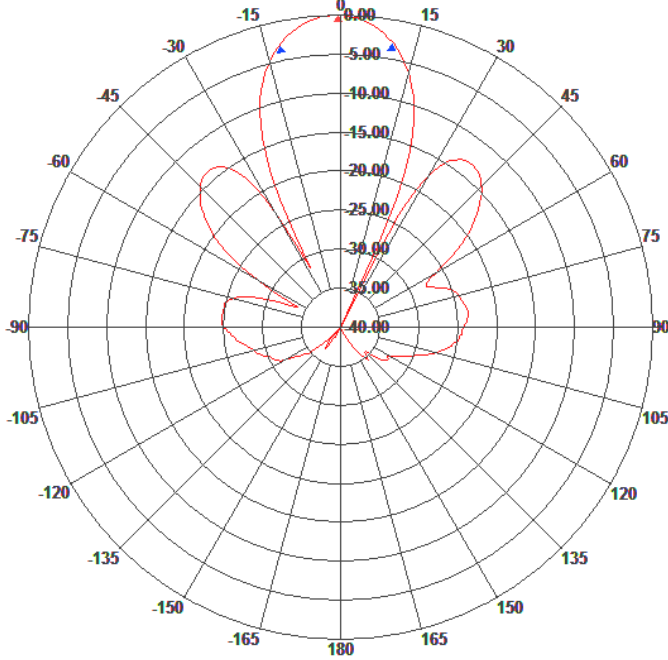
Azimuth Pattern
