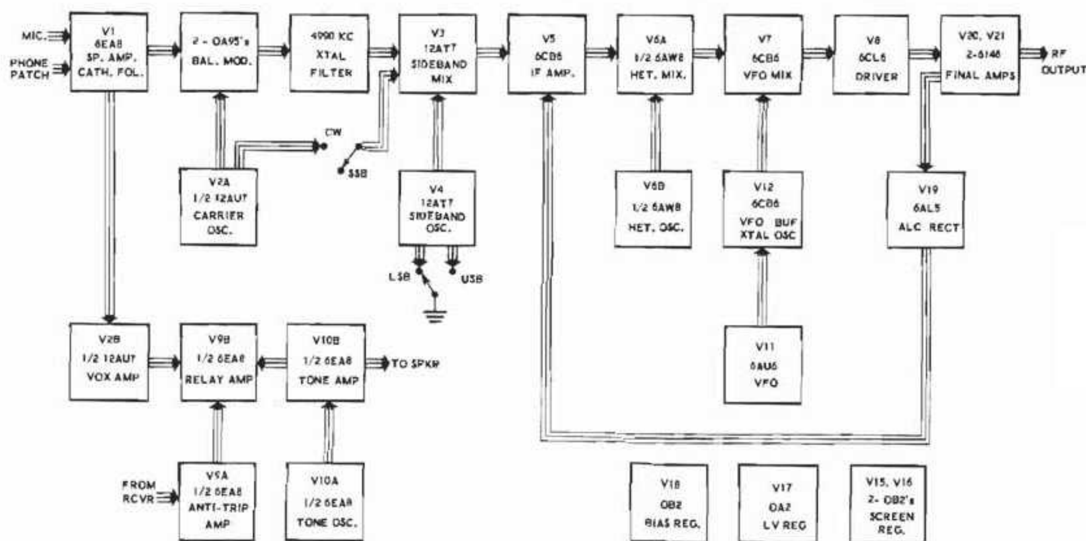
BLOCK DIAGRAM
