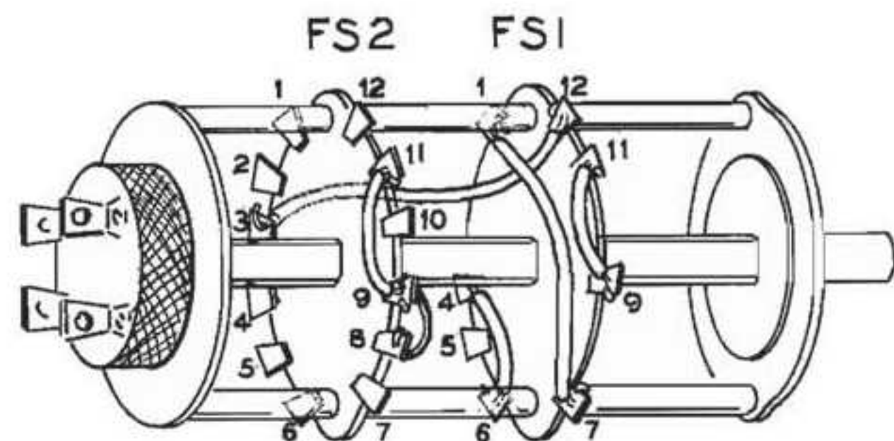
SWITCH FS Detail 40A
