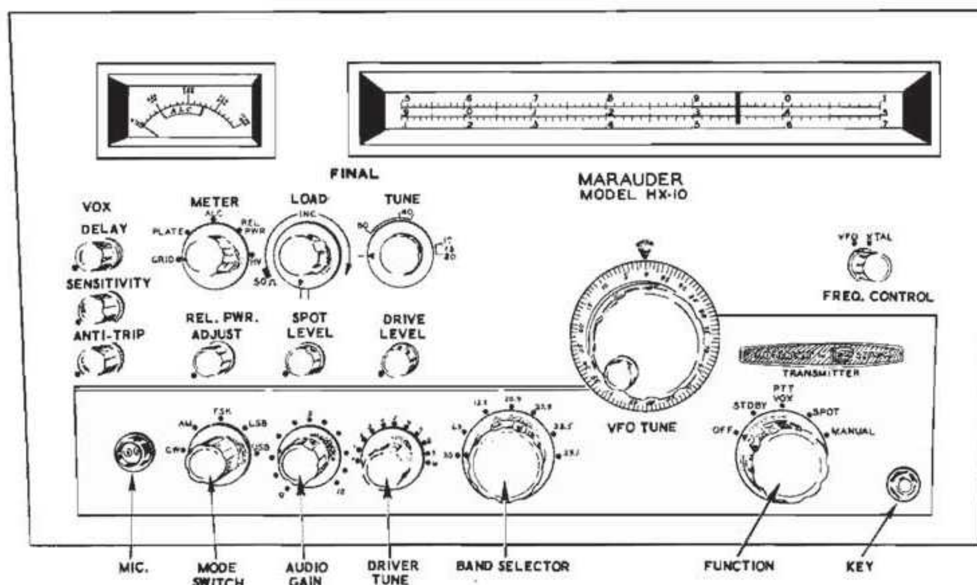
FRONT PANEL CONTROLS
